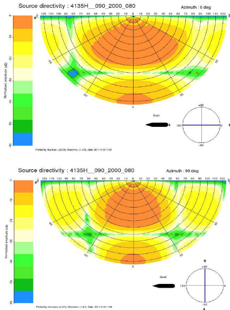
Figure 2.3: Directivity plots in the vertical plane for a 4135 in 3 array source with an azimuth of (a) 0 degrees (inline; front to back of vessel) and (b) 90 degrees (crossline; port to starboard of vessel) at frequencies 0-100 Hz.
