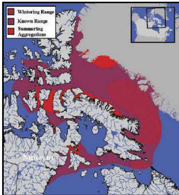
Figure 3.1: Narwhal distribution in Baffin Bay ( www.dfo-mpo.gc.ca ).
