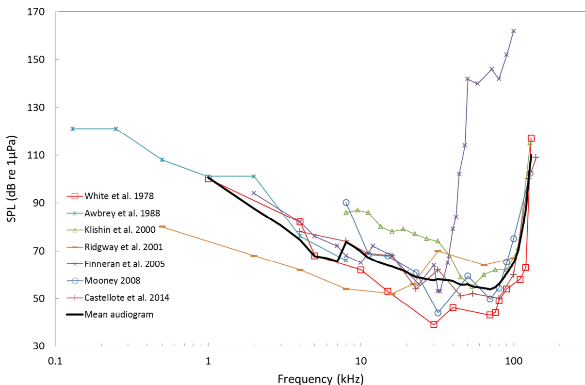
Figure 4.1: Summary of audiograms measured from beluga whales; all are from captive animals except the audiogram presented by Castellote et al. 2014. A mean audiogram for all measurements is shown as a black line; this mean audiogram does not include those values presented by Finneran et al. (2005) as this individual was thought to be suffering from hearing loss due to an aminoglycoside antibiotic treatment.
