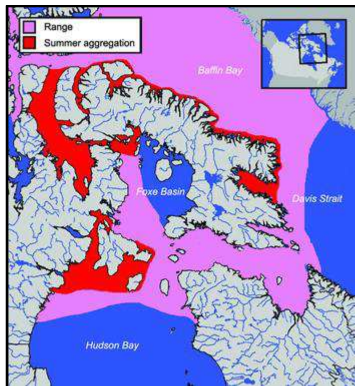
Figure 3.3: Bowhead whale distribution, Eastern Canada / Western Greenland population ( www.dfo-mpo.gc.ca ).
