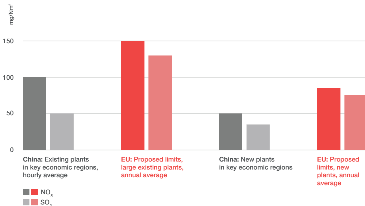
Figure 6: Comparing SO 2 and NO x regulation in the EU and China.
